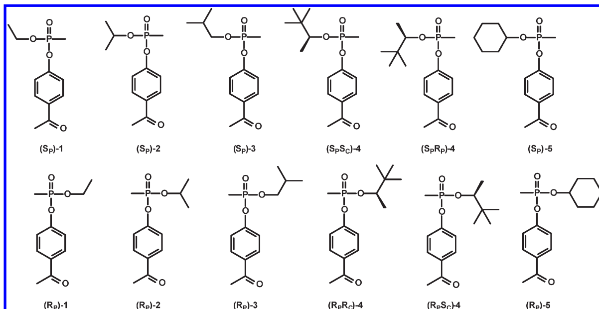
Scheme 3: Structures of Organophosphate Substrates
